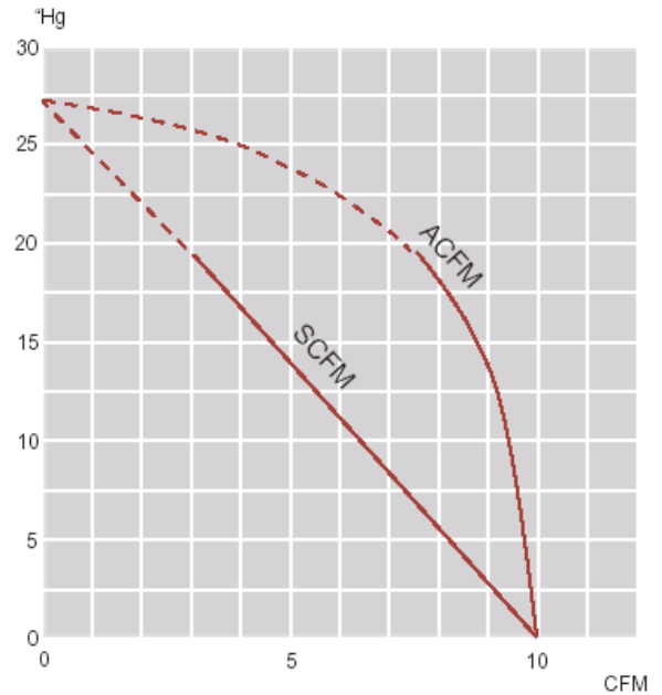
Performance Curves: 60Hz Vacuum
