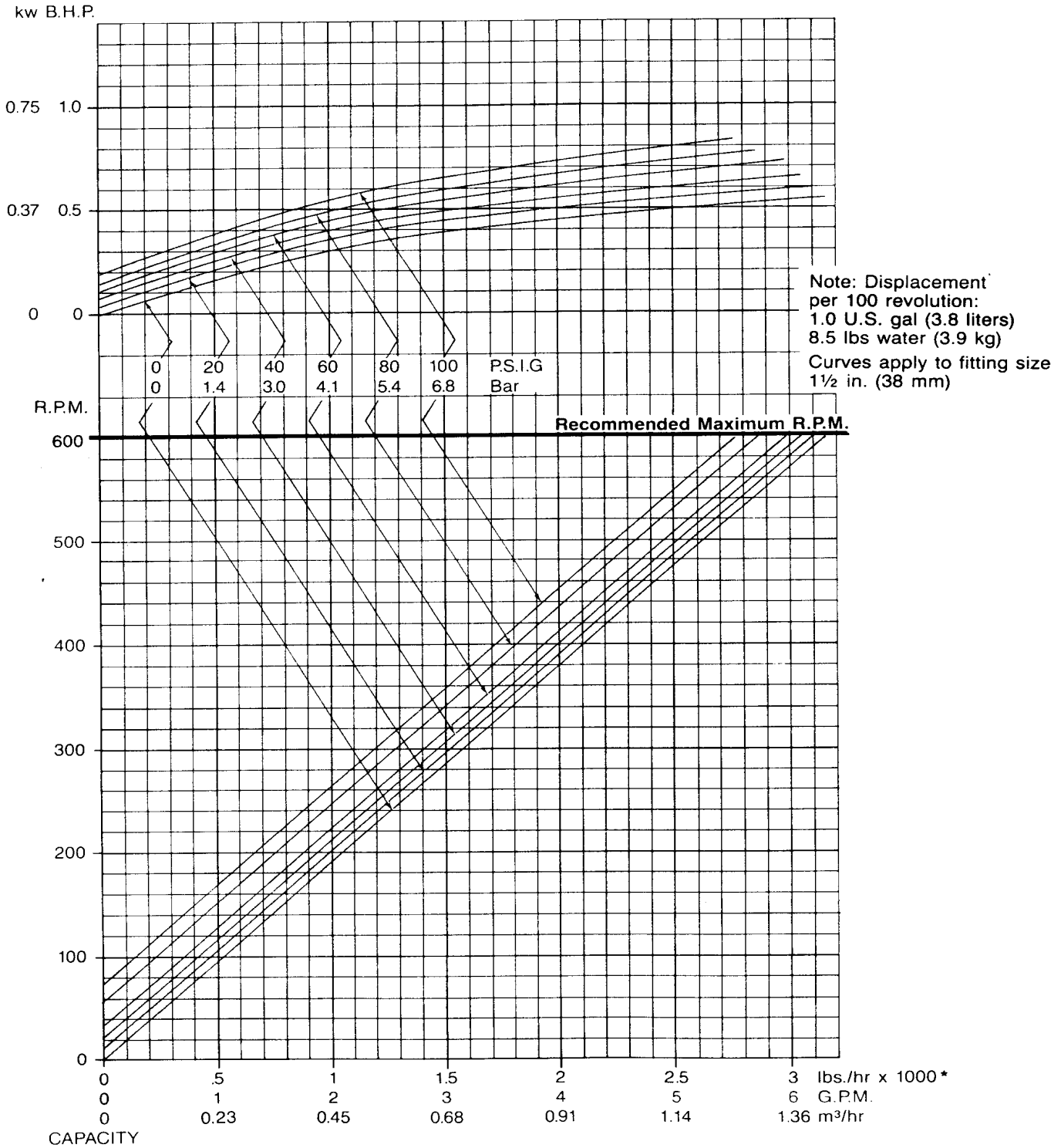
MODEL NO. 1 ROTARY PUMP CAPACITY CURVE
