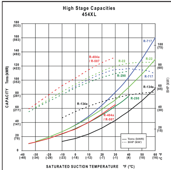
Figure 1 High-Stage Capacities
