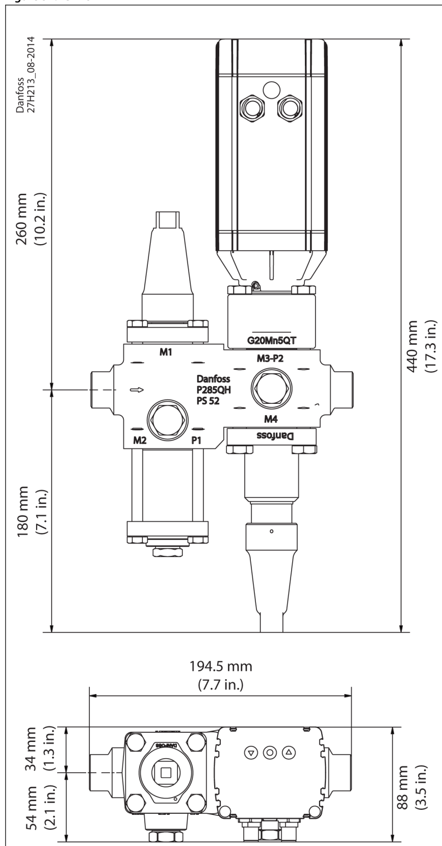
Figure 51: ICF 15-4
