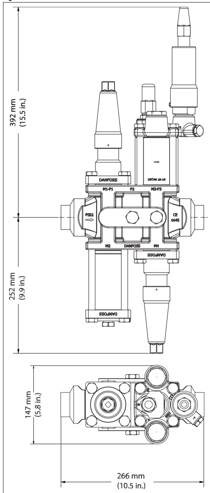
Figure 57: ICF 25-4
