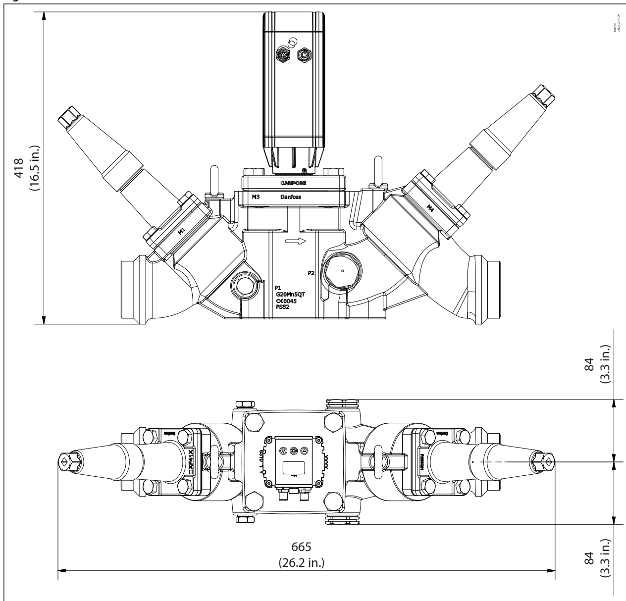
Figure 60: ICF 65-3
