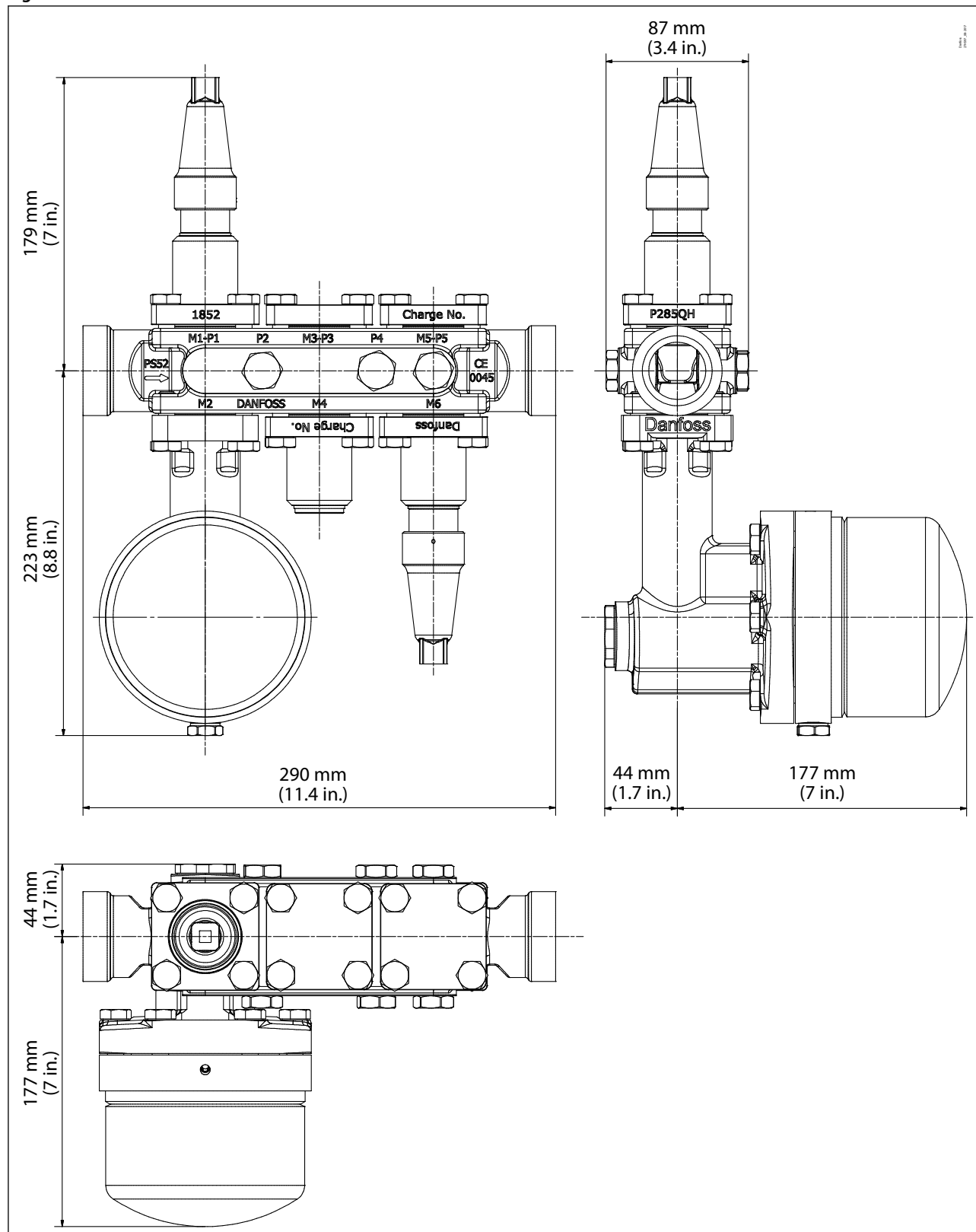
Figure 55: ICF 20-6
