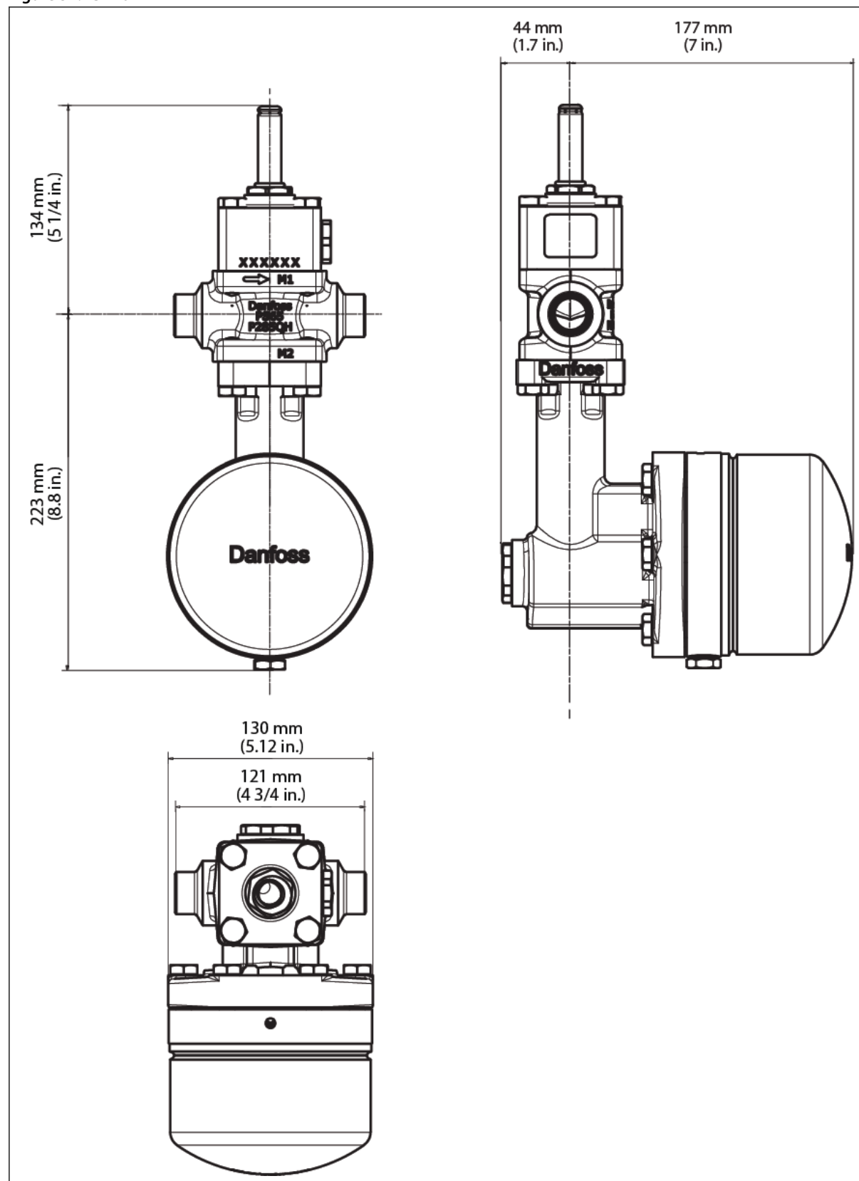
Figure 52: ICF 20-2
