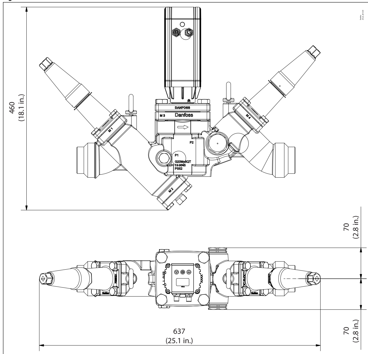
Figure 59: ICF 50-4
