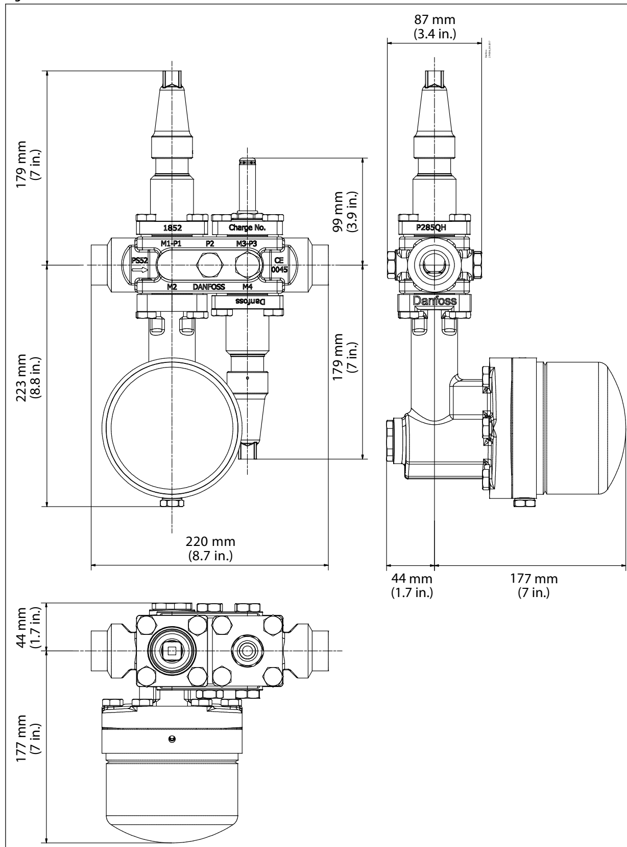
Figure 53: ICF 20-4
