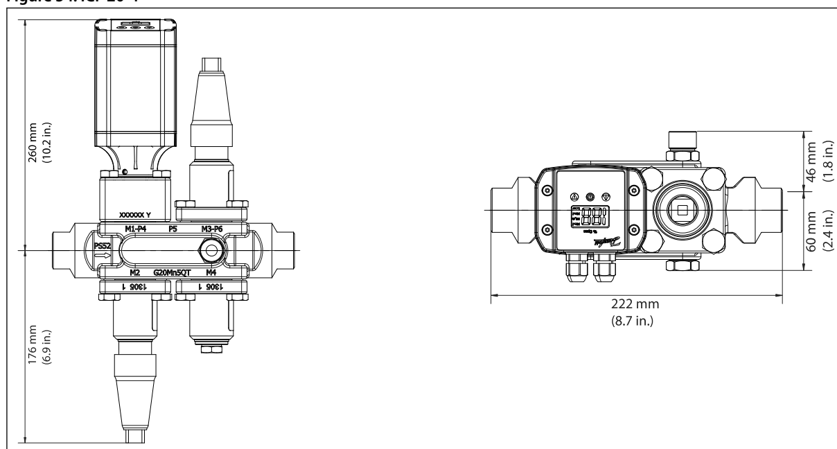
Figure 54: ICF 20-4
