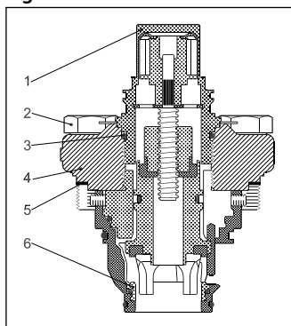
Figure 33: ICM 25-A or B motor operated valve module
