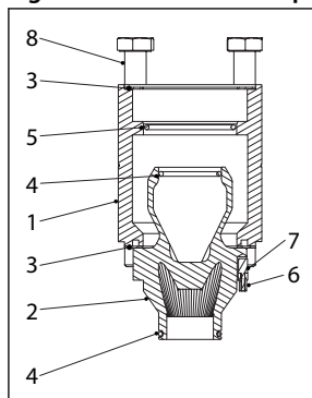
Figure 36: ICFG 25 Pilot-operated valve module
