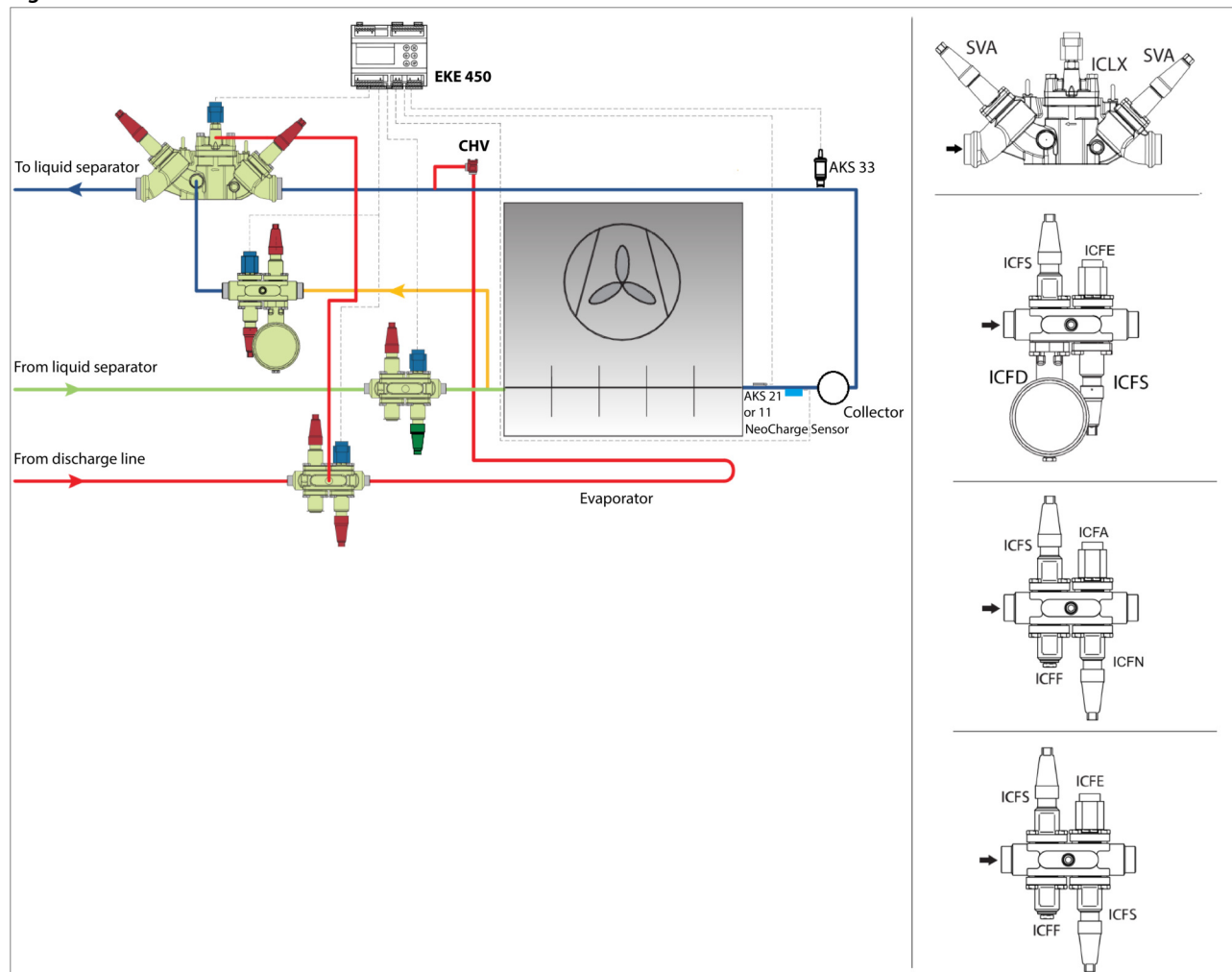
Figure 6: CCR Controlled Circulation Rate
