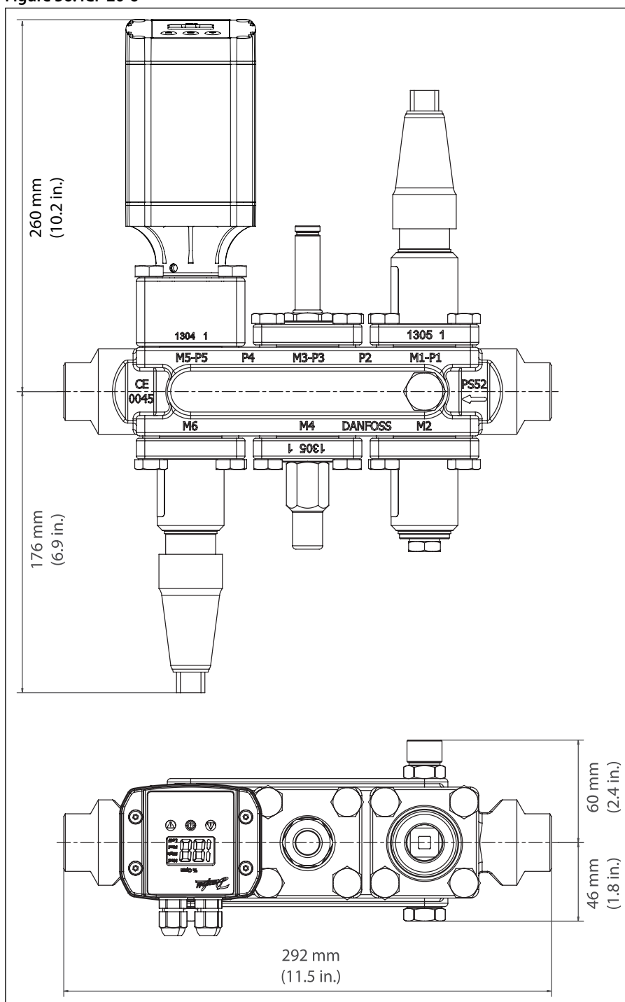
Figure 56: ICF 20-6
