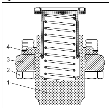
Figure 31: ICFC 25 check valve module
