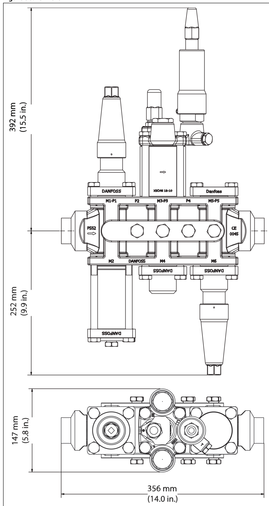
Figure 58: ICF 25-6
