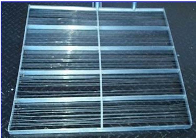
Stainless Steel Cutter. Dimensions: 35 in. x 32 in. and shaft: 17 in. H. 10 divisions each one with 17 cables in horizontal, 3/8 of clearance, missing 10 cables. Overall dimension: 35 in. L x 32 in. W x 17 in. H.
