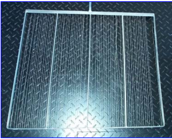
Stainless Steel Cutter. Dimensions: 29-1/2 in. x 26 in. and the shaft: N/A. 4 divisions each one with 15 cables, 3/8 of clearance, missing 8 cables. Overall dimension: 29-1/2 in. L x 26 in. W x 3 in. H.
