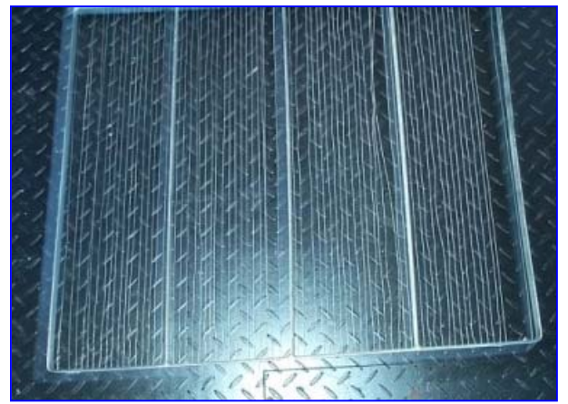
Stainless Steel Cutter. Dimensions: 29-1/2 in. x 26 in. and the shaft: N/A. 4 divisions each one with 15 cables, 3/8 of clearance, missing 8 cables. Overall dimension: 29-1/2 in. L x 26 in. W x 3 in. H.
