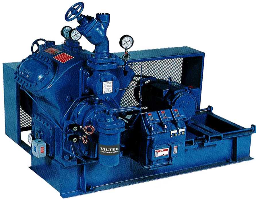
4-cylinder 440 VMC V-belt booster unit
