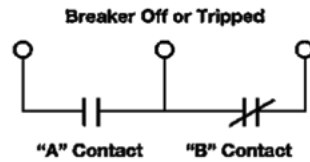
Auxiliary Switch Wiring Diagram
