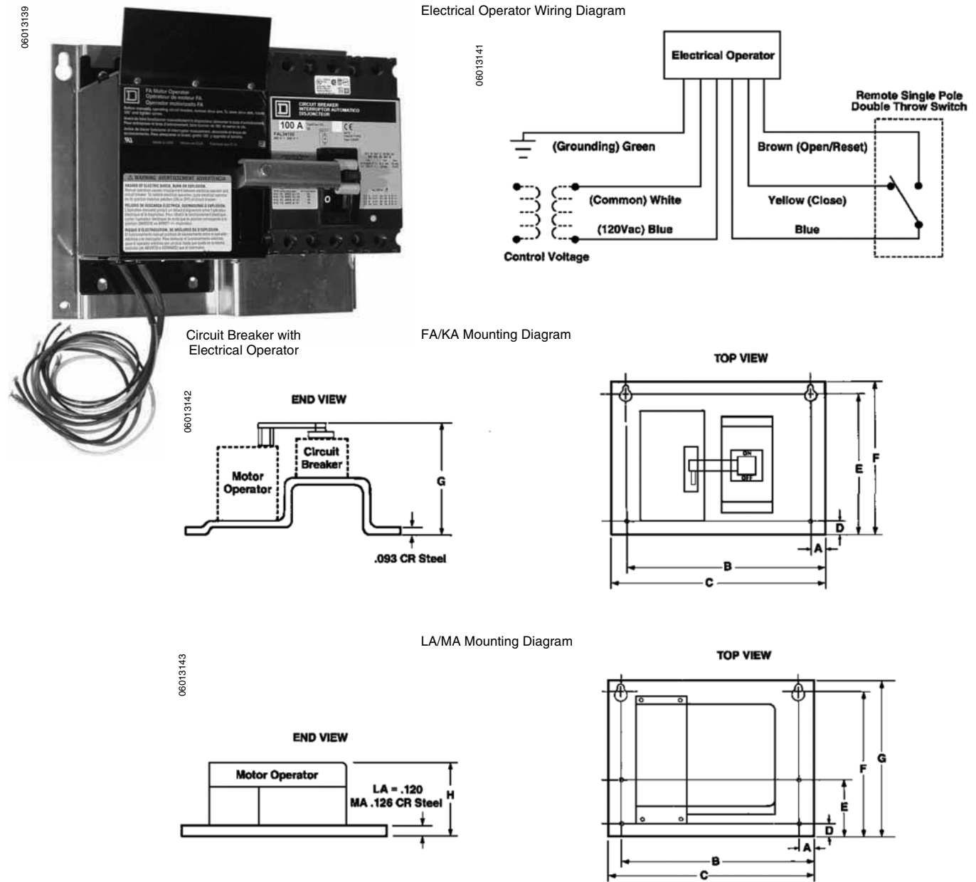
Figure 24: Electrical Operator Side Mount Dimensions and Wiring Diagram
