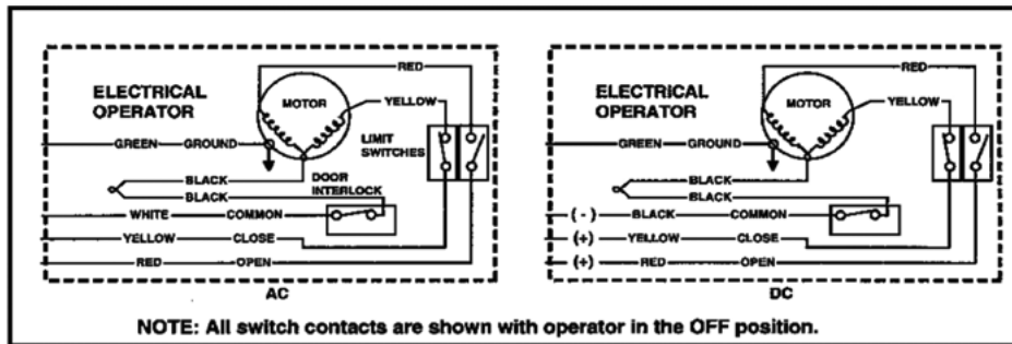
Internal Schematic
