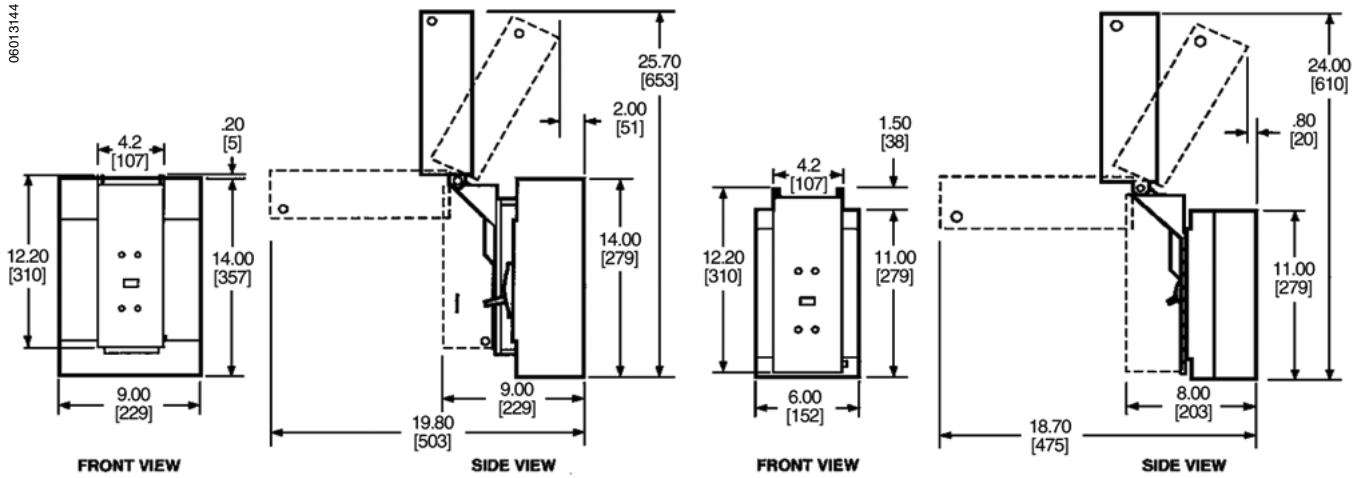
Figure 25: Top Mount Electrical Operator Dimensions and Wiring Diagrams
