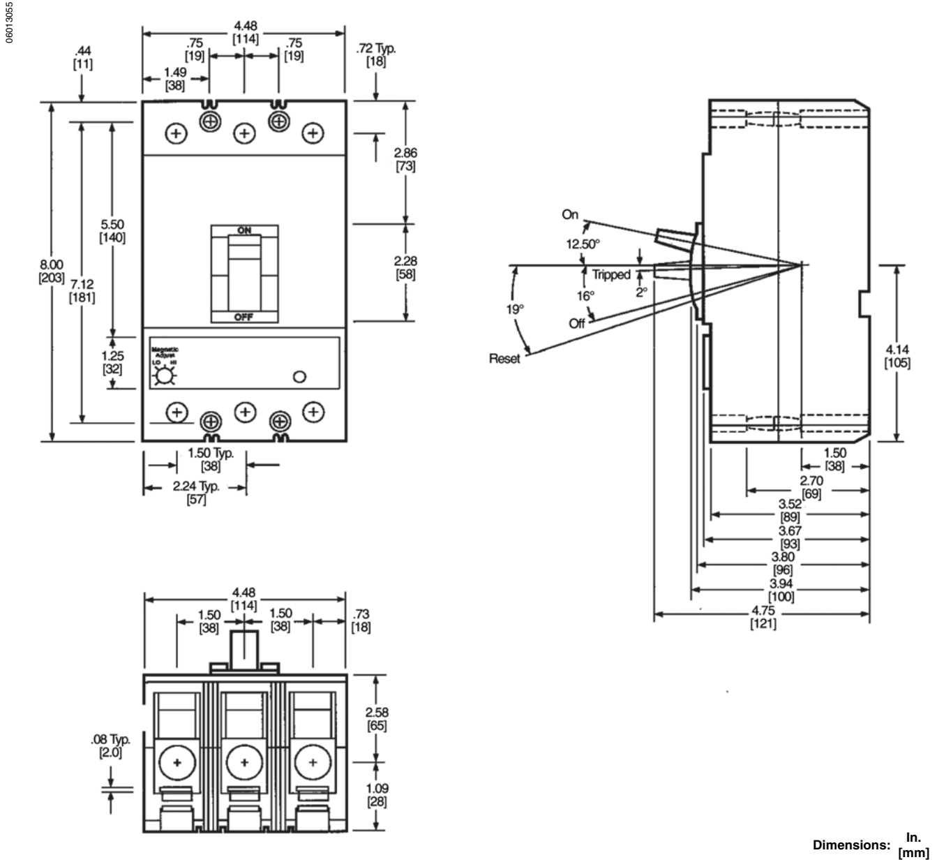
Figure 13: KAL, KHL, KCL, KIL 250 Ampere Frame
